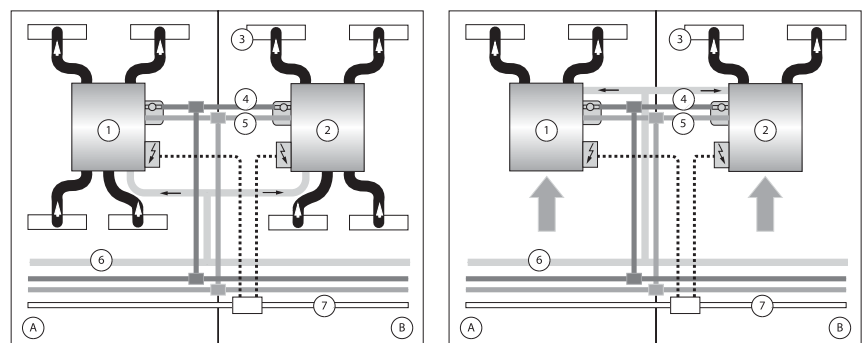
Figure 1 - Typical installations
