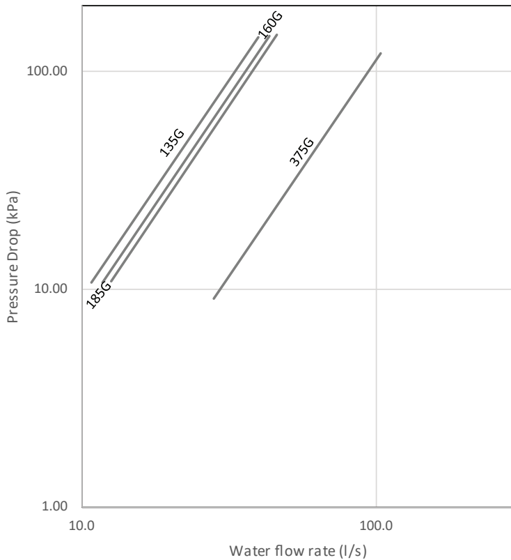
GVWF G - Evaporator pressure drop
