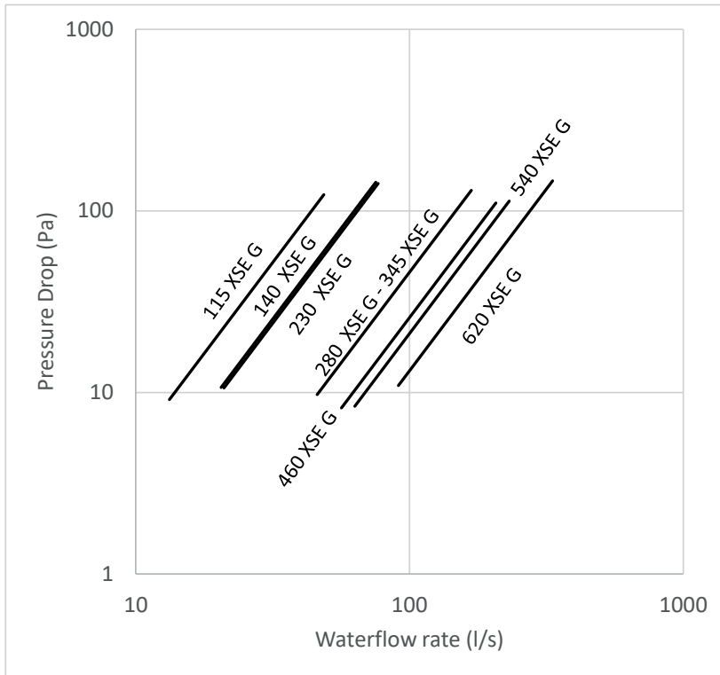
GVWF G - Condenser pressure drop
