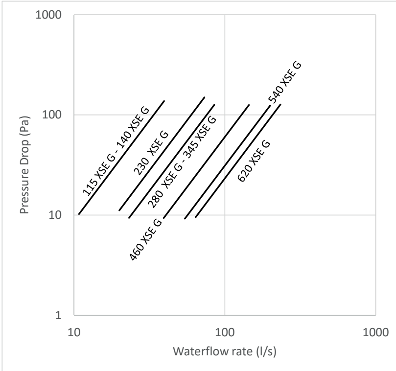
GVWF G - Evaporator pressure drop
