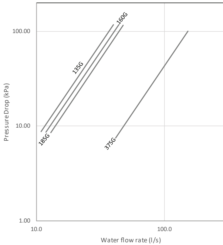
GVWF G - Condenser pressure drop
