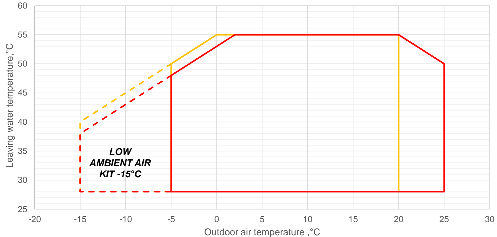
CXB - HEATING MODE
