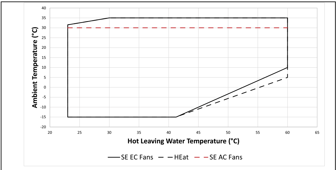
Figure 15 – CXAF Heat pump operating map
