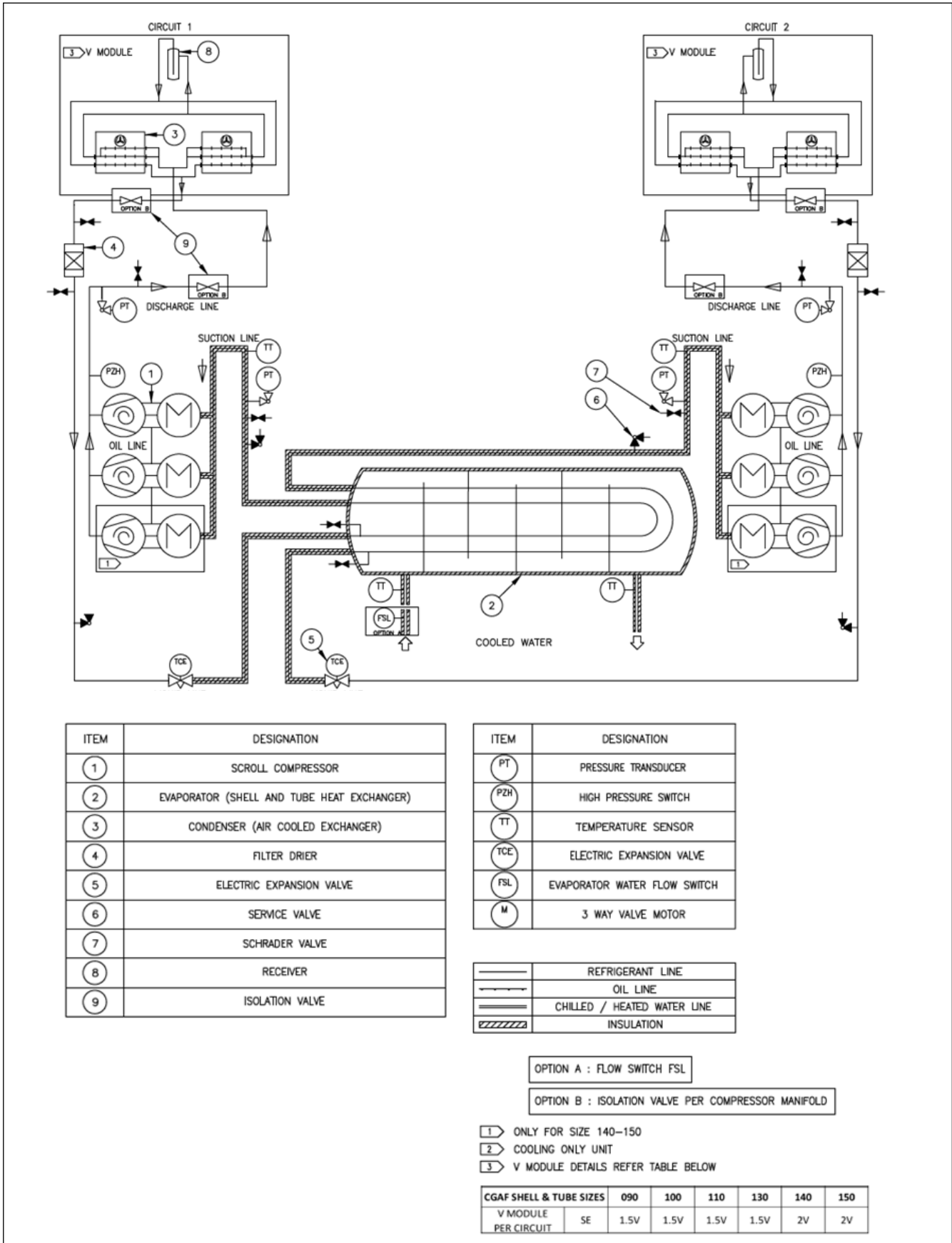
Figure 10 – Example of typical refrigerant system schematic and oil lube circuit schematic for CGAF S and T
