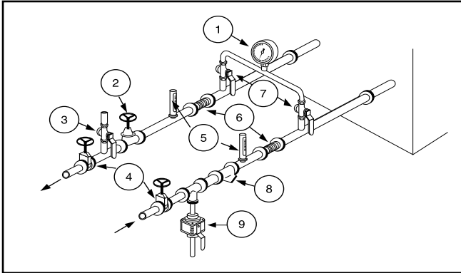
Figure 4 – Unit typical water circuit
