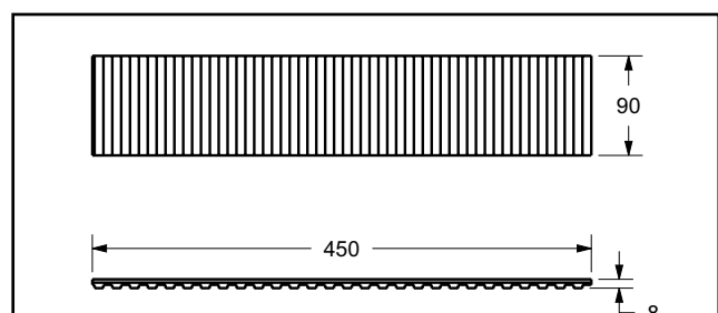
Figure 3 – Isolator pads
