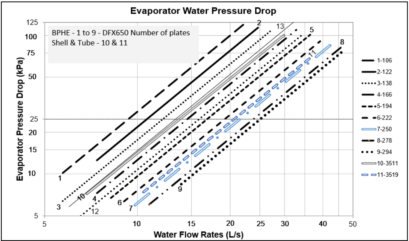
Figure 5 – CGAF / CXAF Evaporator water pressure drop (BPHE, Shell and Tube)
