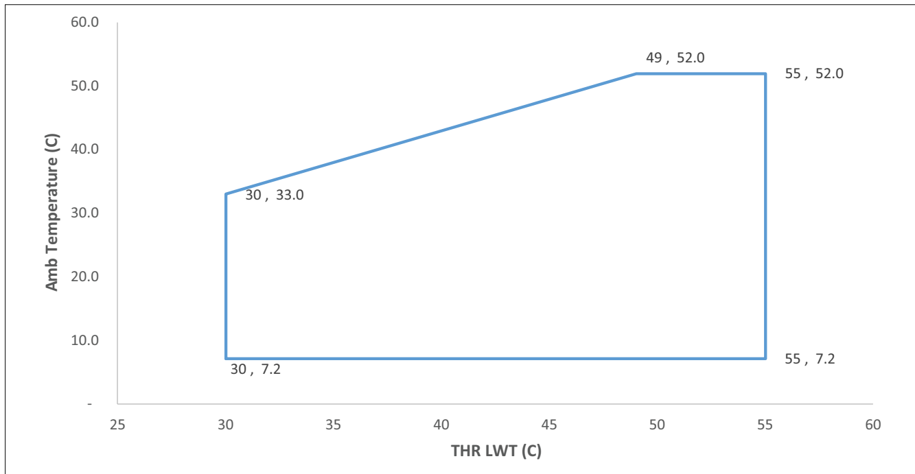
Figure 17 – Total heat recovery operating map
