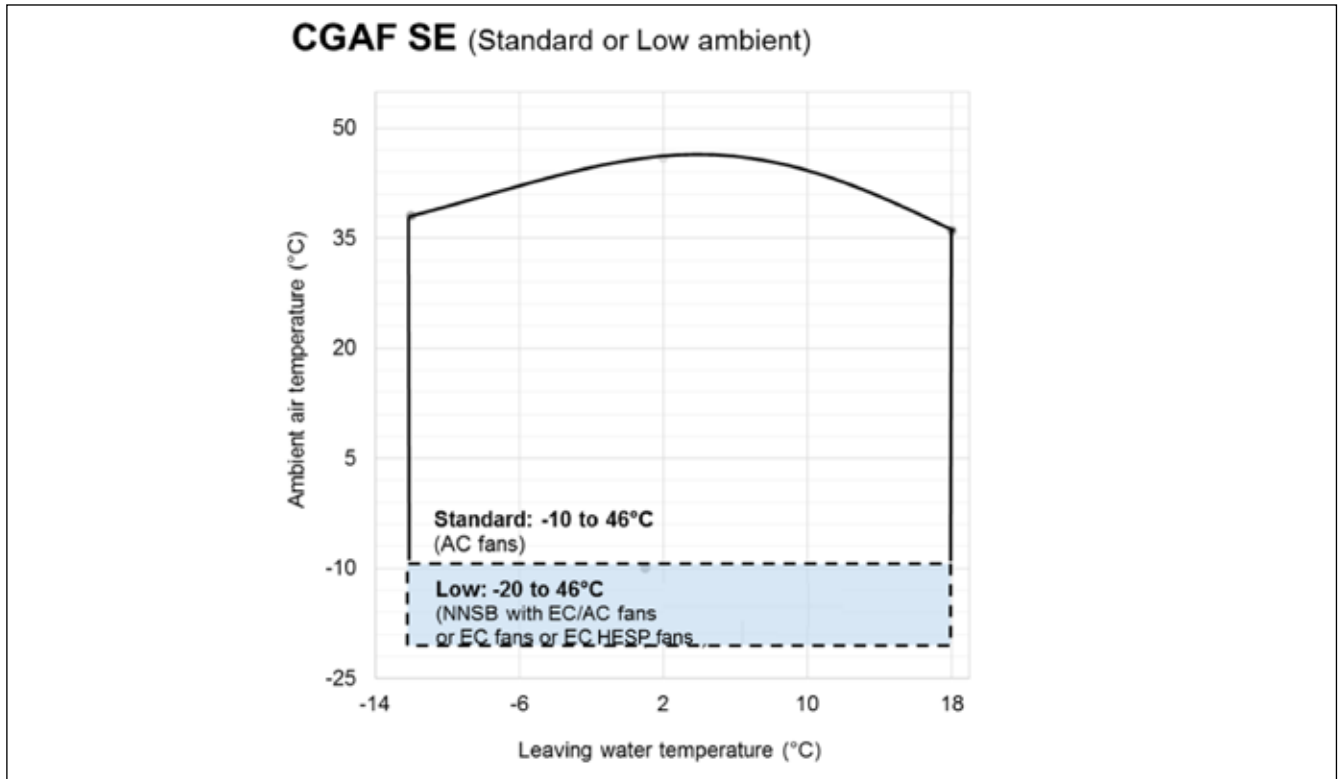
Figure 13 – Operating map for CGAF / CXAF
