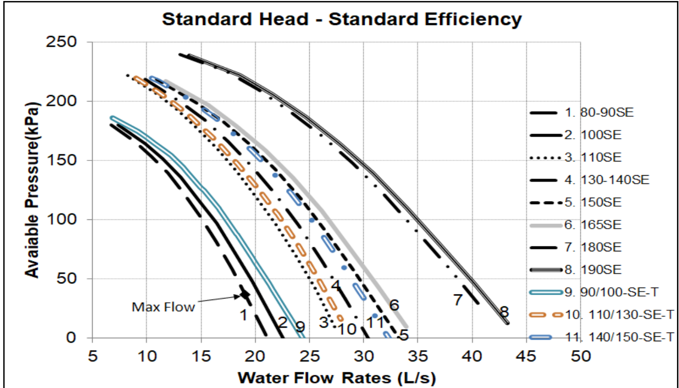
Figure 6 – Pump curve - Sizes 090-190 –Standard / High Head - BPHE / Shell and Tube evaporator
