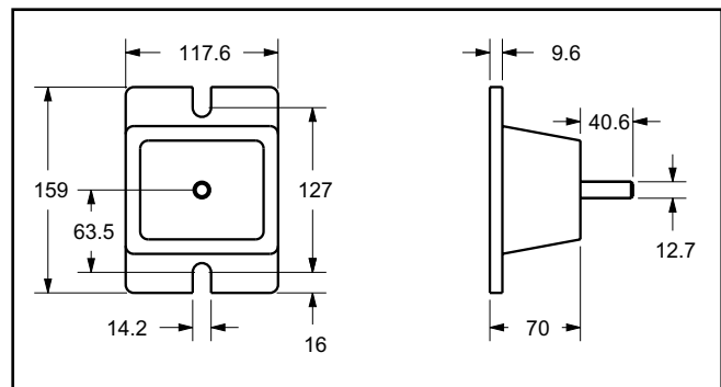
Figure 2 – Elastomeric isolator
