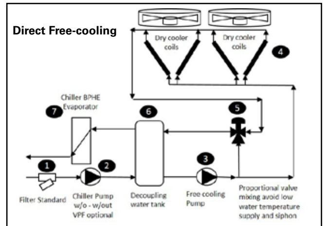
Figure 23 – Schematic – Free-cooling option
