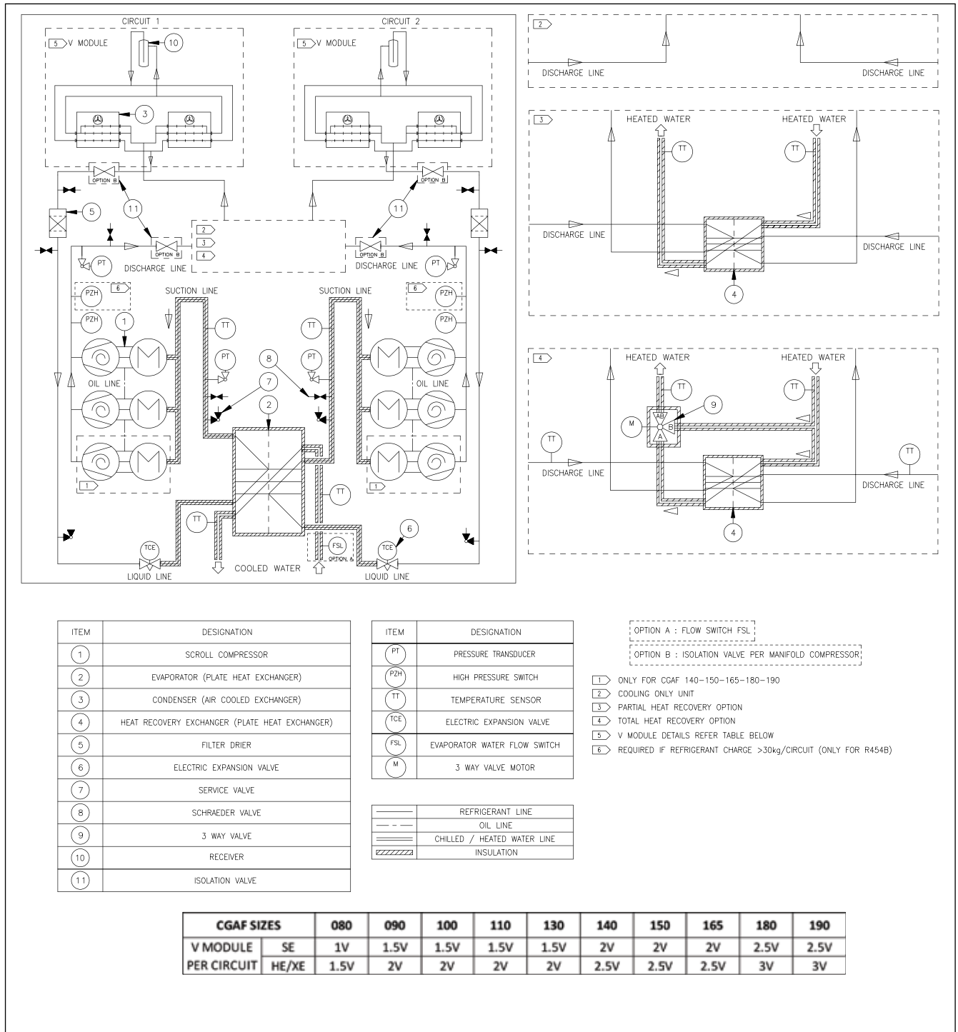
Figure 9 – Example of typical refrigerant system schematic and oil lube circuit schematic for CGAF - BPHE
