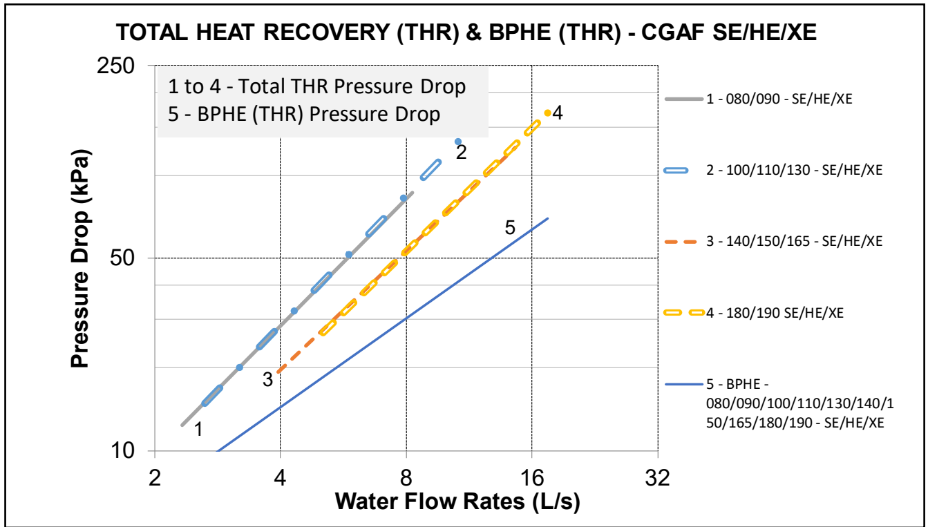
Figure 18 – Total heat recovery water loop pressure drop total THR and BPHE (THR) curve
