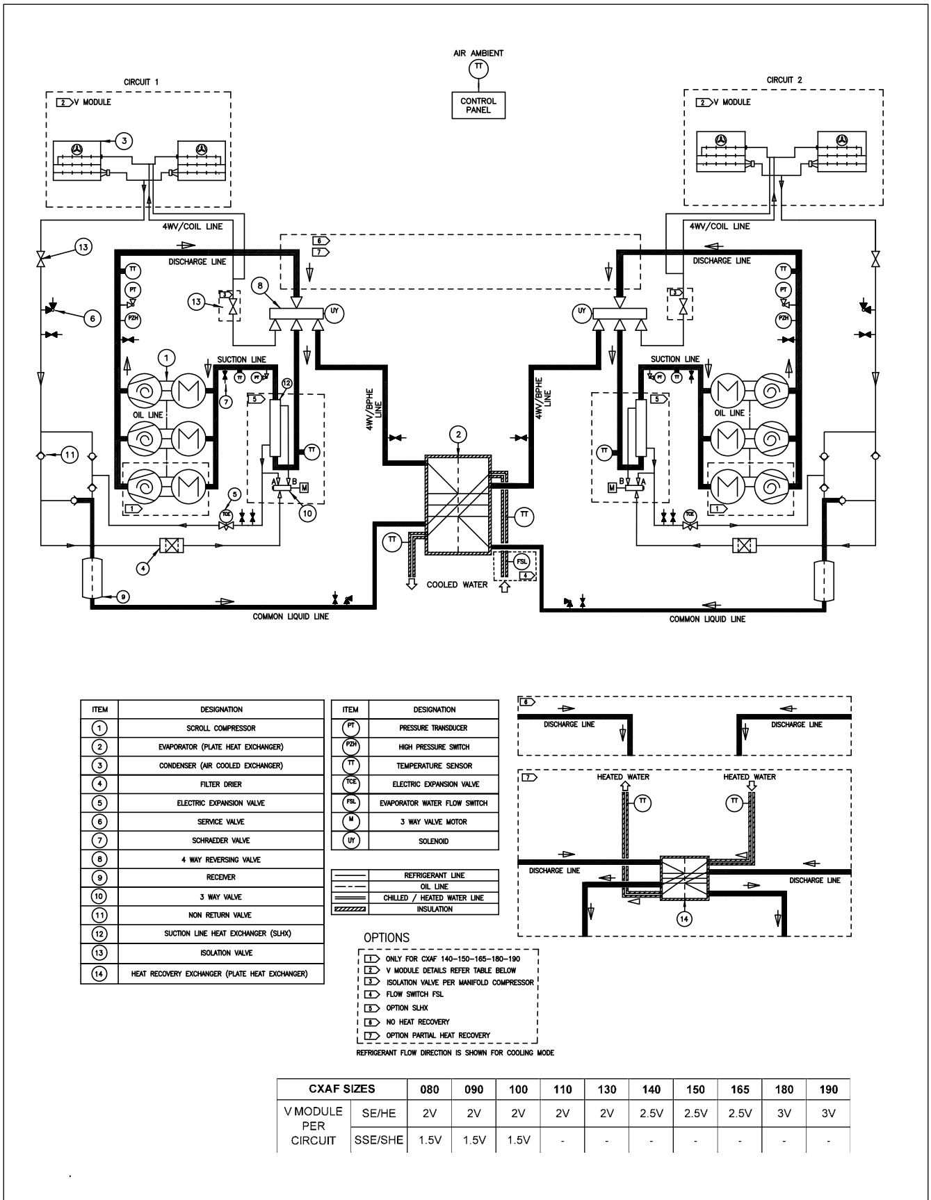
Figure 11 – Example of typical refrigerant system schematic and oil lube circuit schematic for CXAF - BPHE
