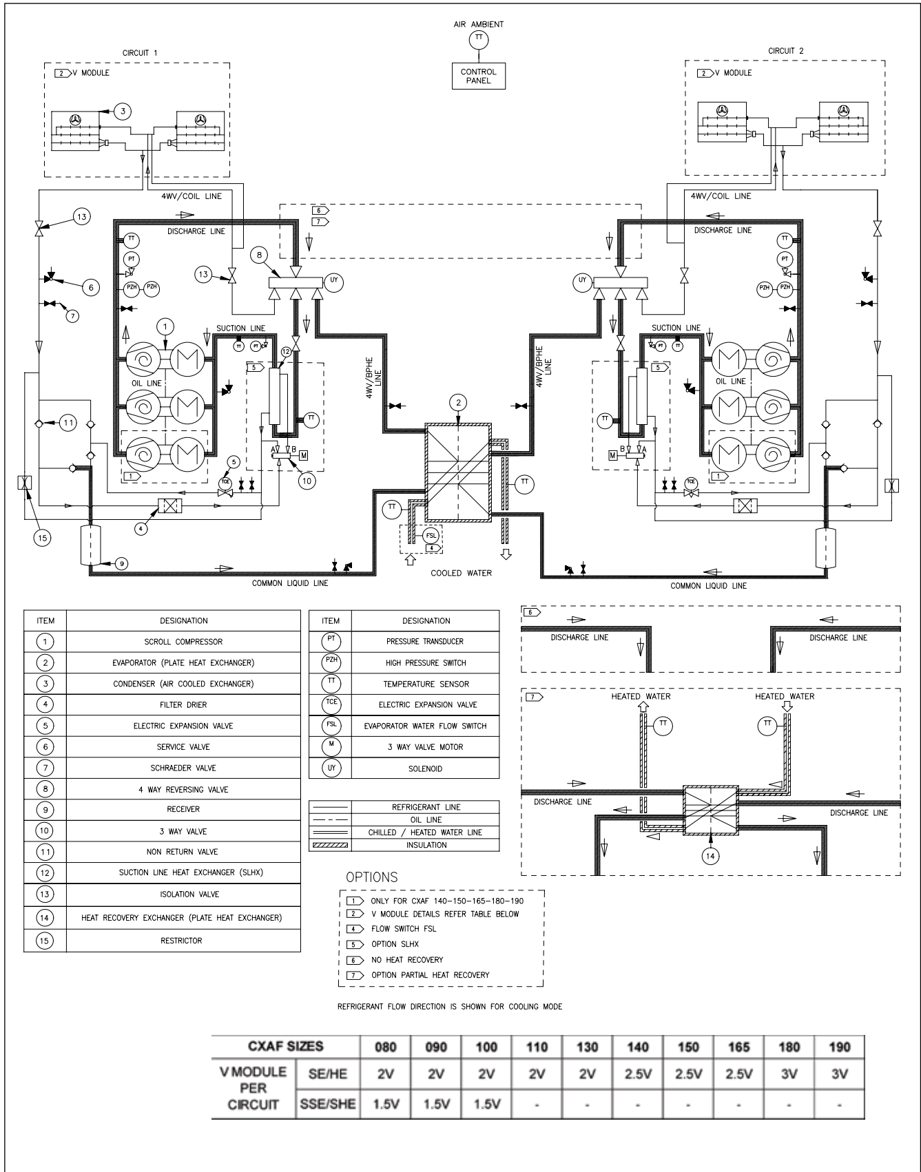
Figure 12 – Example of typical refrigerant system schematic and oil lube circuit schematic for CXAF Heat
