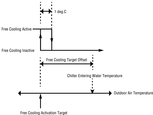
Figure 22 – Free-cooling enabling conditions
