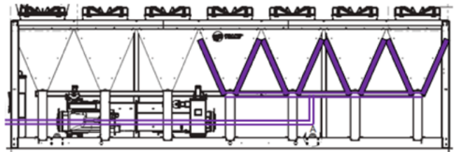
b. Partial Free Cooling, Direct free cooling version
