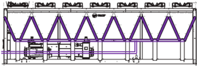
a. Total Free Cooling, Direct free cooling version
