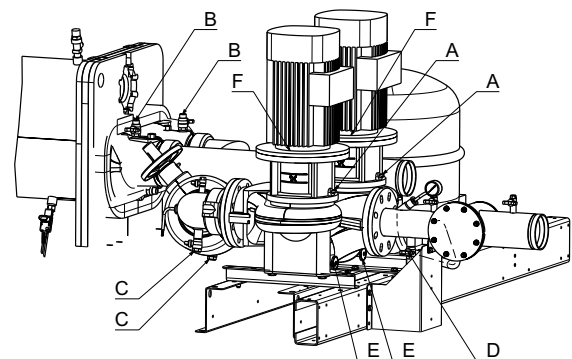
Figure 36 – Pump Package
